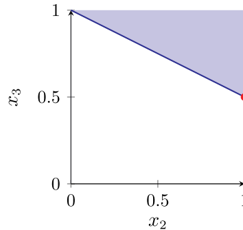
Figure 1. (Color online) Inequality x_1 + x_2 + 2x_3 \geq 2 on the Face of the Polytope with x_1 = 0
