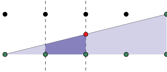
Figure 3. (Color online) Example in Which It Is Impossible to Find a Linear Cut That Separates the Noninteger Vertex (2,0.5) from the Feasible Region
