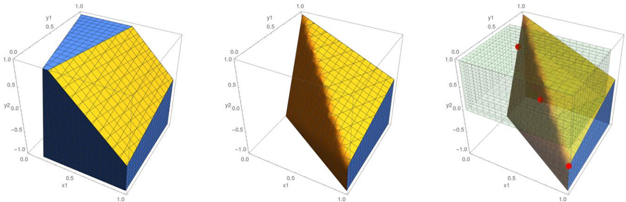
Figure 2. (Color online) Example in Which it is Impossible to Separate the Mixed-Integer Hull from the Infeasible Local Domain
